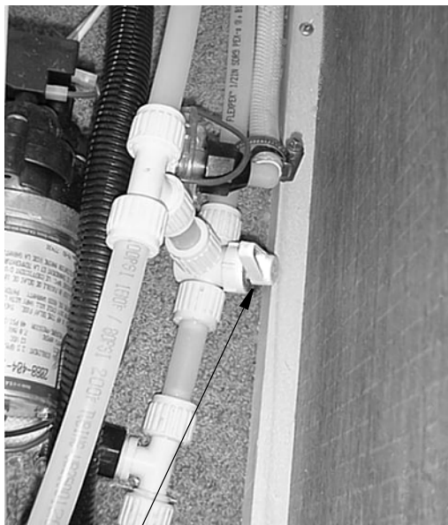
Water Heater Bypass Valve (Typical)
