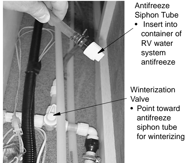
Antifreeze Siphon Tube and Winterization Valve -Typical View
