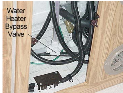
Typical Installation
