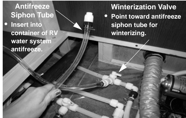
Antifreeze Siphon Tube and Winterization Valve (See Water System Drain Valve chart at the end of this section for location on your coach)
