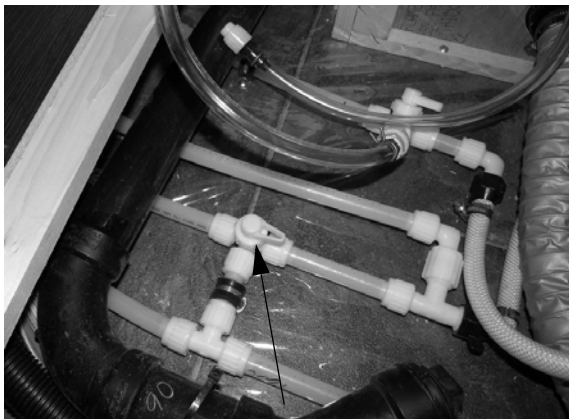
Water Heater Bypass Valve (See Water System Drain Valve chart at the end of this section for location on your model)
