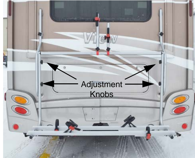
Bike Rack Turn adjustment knobs to remove bike rack and adjust up or down. Insert adjustment knobs and fully tighten. -Typical View
