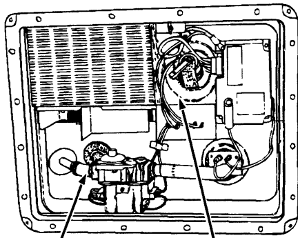
Drain Plug P-T Relief Valve WATER HEATER OUTSIDE ACCESS
