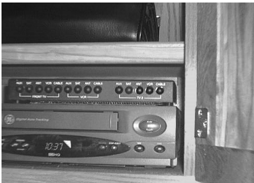
Video Selector System (in right front overhead compartment)
