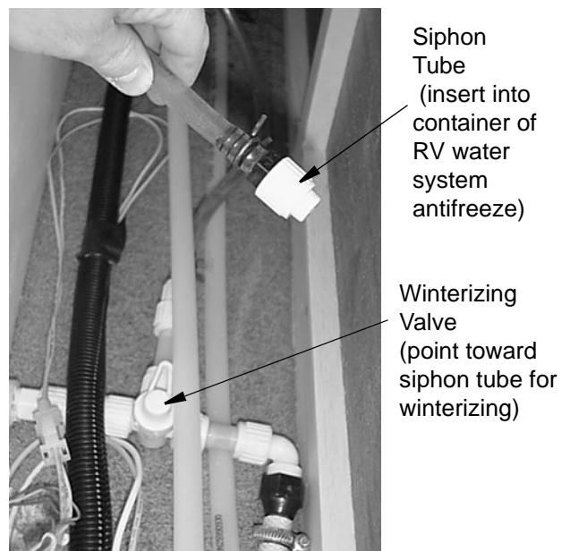
Winterization Valve (See Drain Valve Location chart at end of this section)
